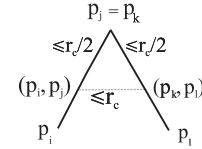
Fig. 4. Primary interference constraint and its effect on the separation distance of the mid-points of the communicating links.
