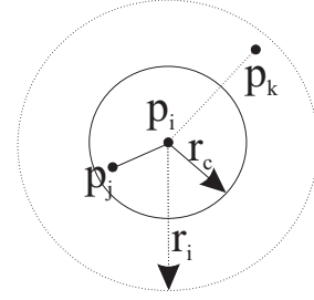
Fig. 1. An illustration of the communication radius and the interference radius . Nodes p_i and p_j ( p_k ) can communicate (interfere) with each other.
