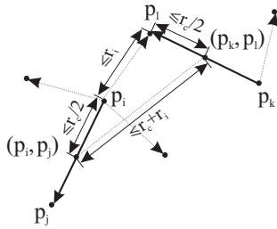
Fig. 5. Secondary interference constraint and its effect on the separation distance of the mid-points of the communicating links.
